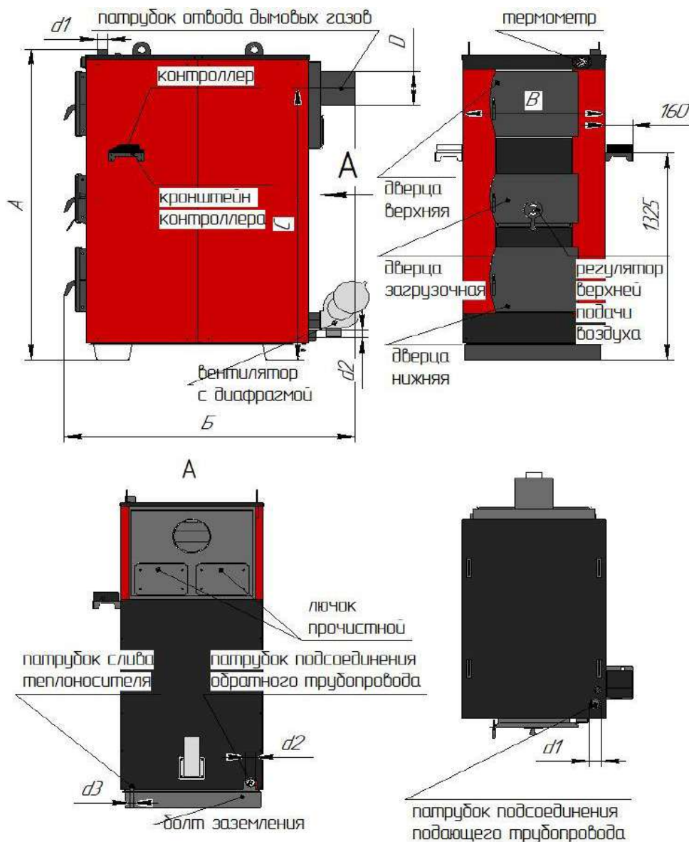
DRAGON SMART 80,100
